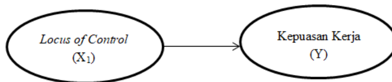
Figure 1. Constellation of Variable X_1 Toward Y
