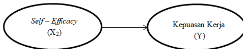
Figure 2. Constellation of Variable X_2 Toward Y
