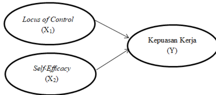
Figure 3. Constellation of Variables X_1, X_2 Toward Y
